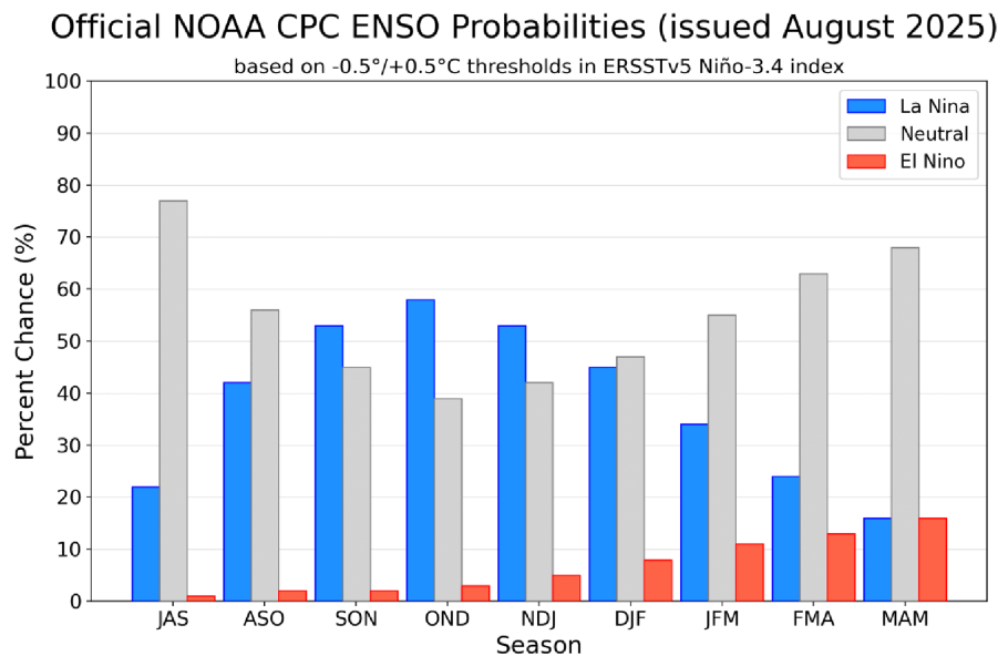
Figure 7. Official ENSO probabilities for the Niño 3.4 sea surface temperature index ( 5^{\circ}\text{N} - 5^{\circ}\text{S} , 120^{\circ}\text{W} - 170^{\circ}\text{W} ). Figure updated 14 August 2025.
